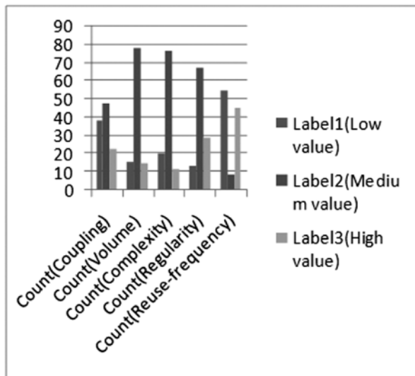
Figure 1.3: Bar Chart of Statistics of the Input Attribute in Data set
