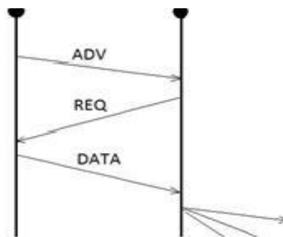
Fig2. Sensor protocol for information via negotiation (SPIN)
