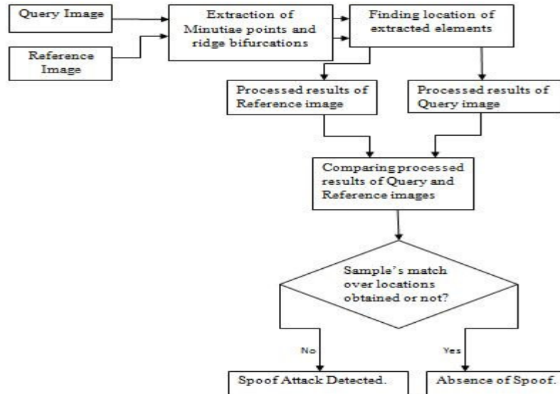
Figure 2: Framework of proposed hybrid fusion method.
